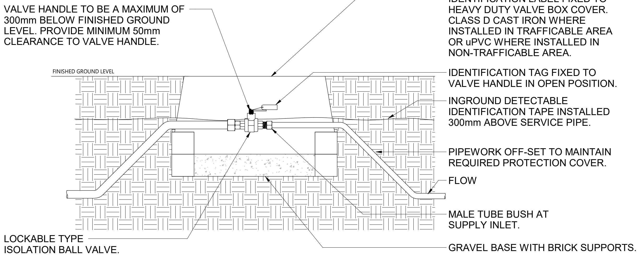
INGROUND ISOLATION VALVE BOX NTS
