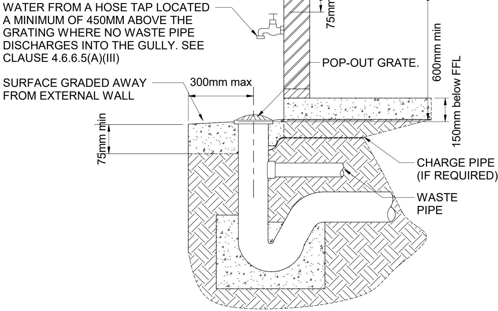
OVERFLOW RELIEF GULLY NTS
